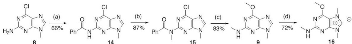
Scheme 4. (a) PhCOCl, pyridine; (b) K 2 CO 3 , MeI, acetone; (c) NaOMe, MeOH; (d) MeI, acetone.
