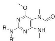
Figure 1. Structures of heteromines A–H.
