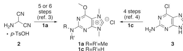
Scheme 1. Previously reported total syntheses of heteromines A and C.
