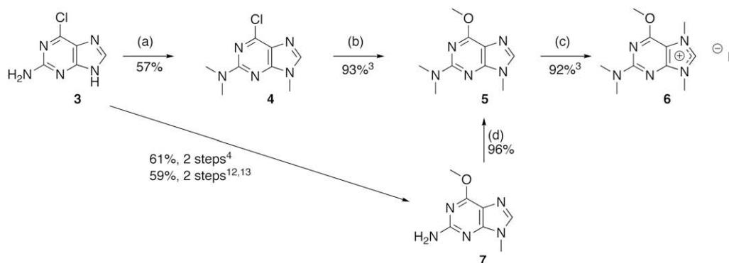
Scheme 2. (a) MeI, NaH, TBAB, THF; (b) NaOMe, MeOH, Δ, see Ref. 3; (c) MeI, acetone, see Ref. 3; (d) HCHO, NaCNBH 3 , AcOH, MeOH, H 2 O.
