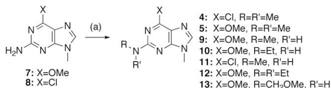
Scheme 3. (a) RCHO, NaCNBH 3 , AcOH, 50 °C, for further details see Table 1.
